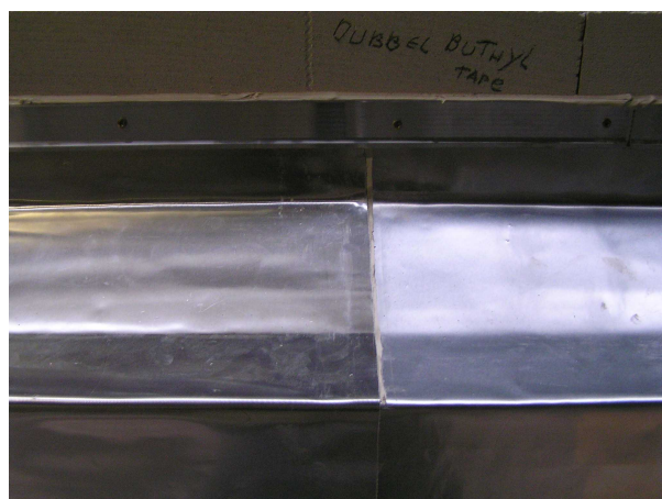
..... or double sided butyl tape. The overlap should be >100mm.
